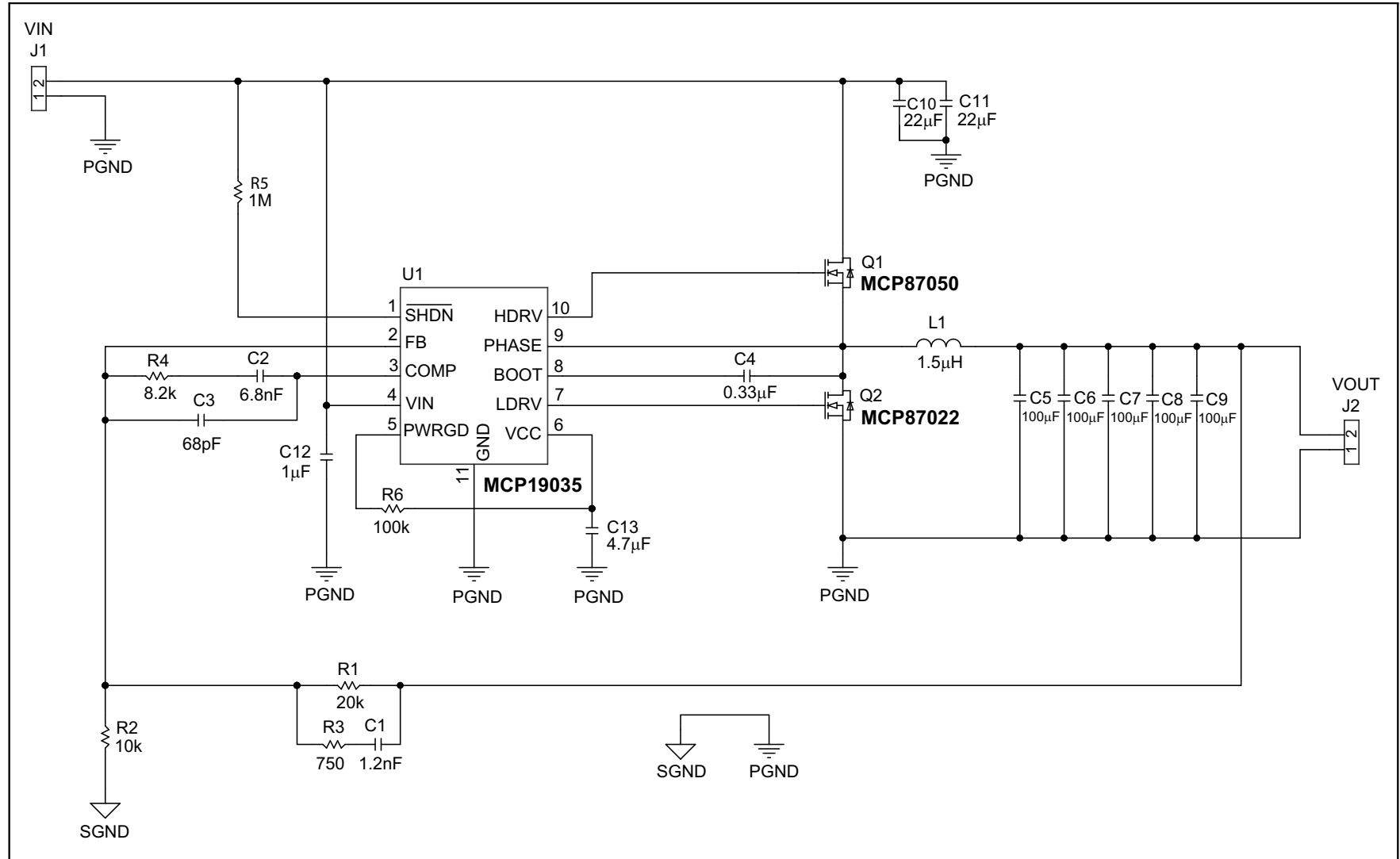
FIGURE 6-4: Schematic Diagram.
