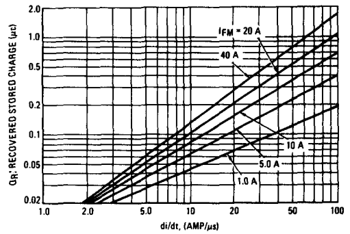
FIGURE 13 – T_J = 75^\circ\text{C}
