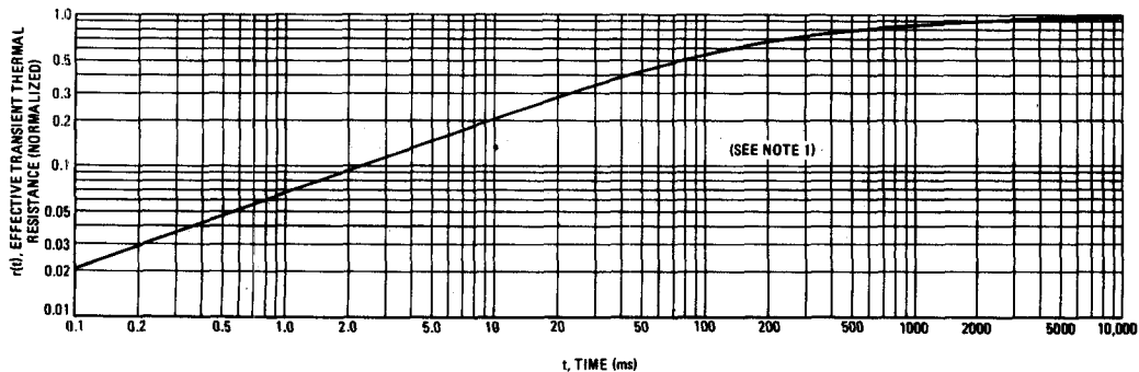
FIGURE 3 – THERMAL RESPONSE
