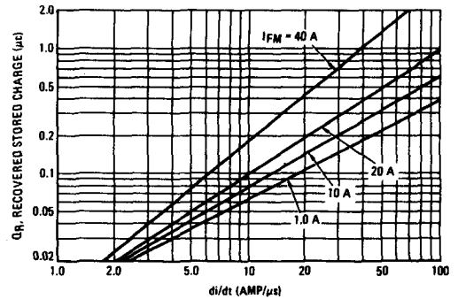
FIGURE 15 – T_J = 150^\circ\text{C}
