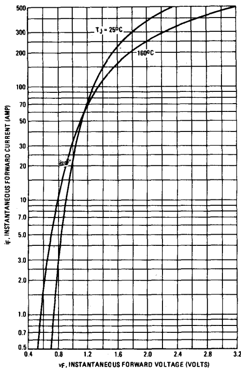
FIGURE 1 – FORWARD VOLTAGE
