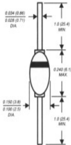
DO-204AP
